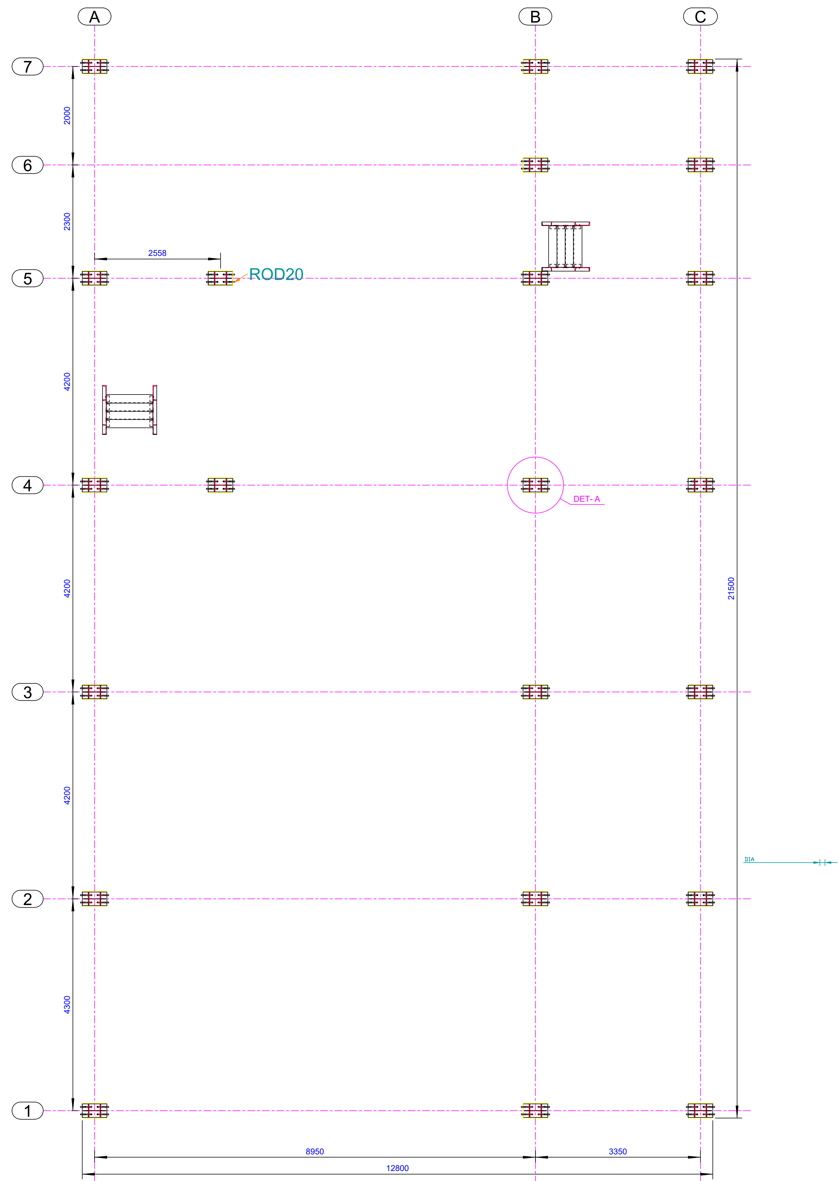
- ANCHOR BOLT PLAN
